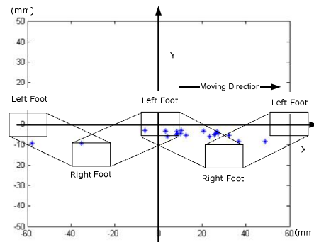
Fig. 2. ZMP trajectories of the learned biped gait
