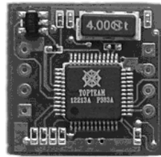
Fig. 5. Photograph of the digital compass.
