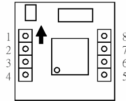
Fig. 6. Structure chart of the digital compass.
