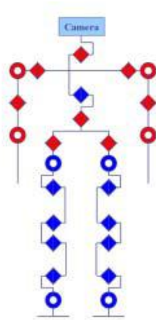
Fig. 1: DOF arrangement of the robot
