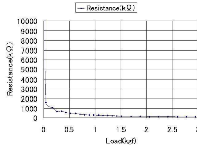
Fig. 3. Characteristic of FlexiForce
