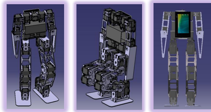
Fig. 3. Bogobot-2 design.
