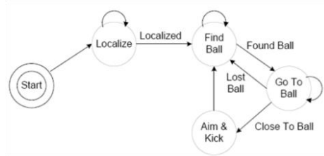
Fig. 7. States based decision algorithm.
