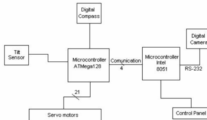
Fig.4.1. Block diagram of the general control system.
