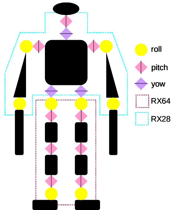
Fig 2. DOF of the robot
