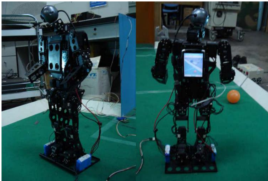
Fig.1. MOS2007 Appearance
