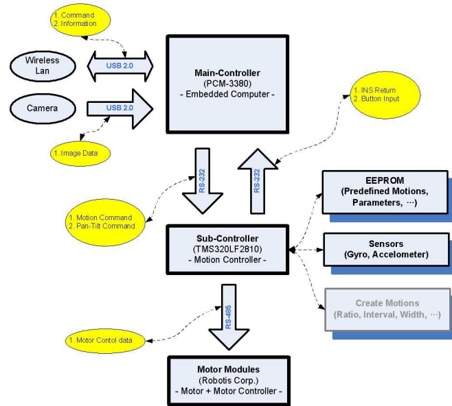
Fig. 2 The software structure of the soccer robot
