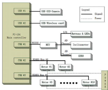
Fig. 2-3. The electrical system architecture of Stepper_Kid
