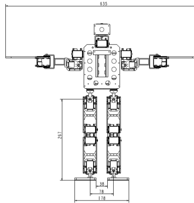
Fig. 2-2. Dimensions of Stepper_Kid
