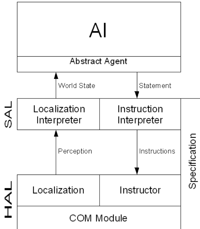
Fig. 3. Software Architecture
