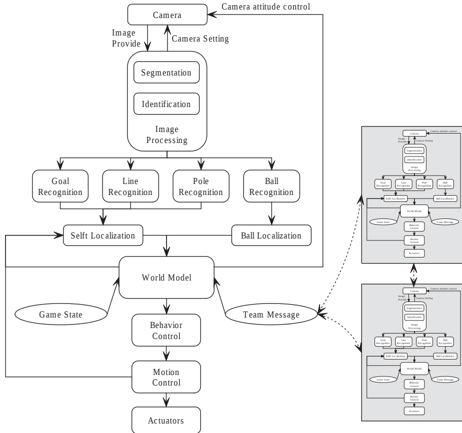
Figure 4: Software Architecture
