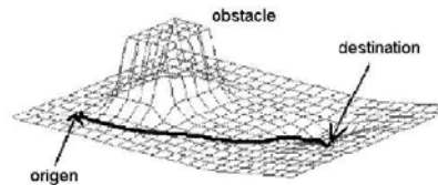
Fig. 3. Example of Potential Field
