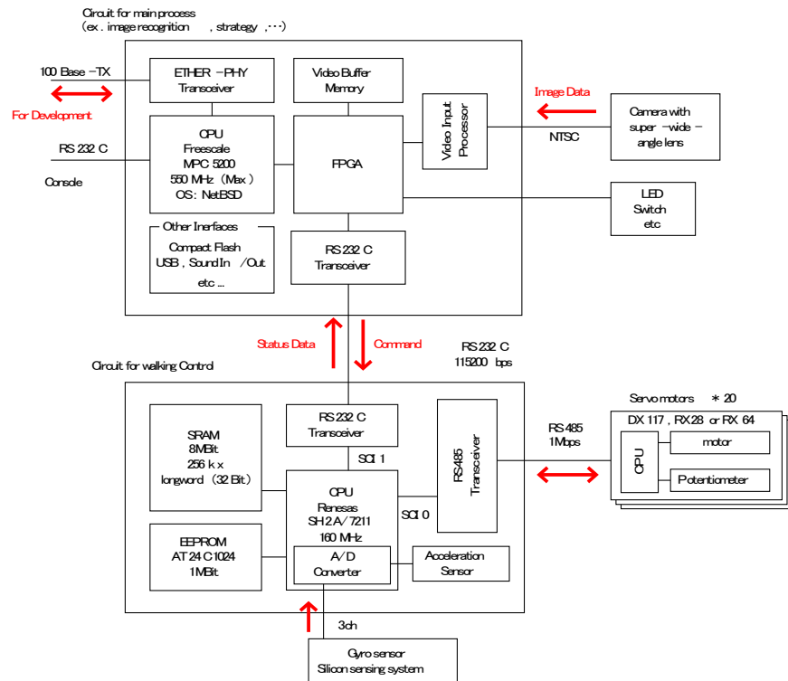
Fig.2 Overview of the Control System
