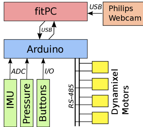
Fig. 2. Electronics architecture
