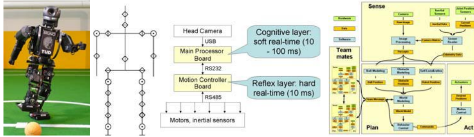
Fig. 1. Autonomous humanoid robot Bruno (with designed head) kicking a ball (left), kinematical robot structure (middle left), main layers of information processing (middle right) and control architecture (right).
