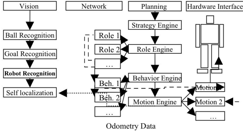
Fig. 1. Structure of the control software
