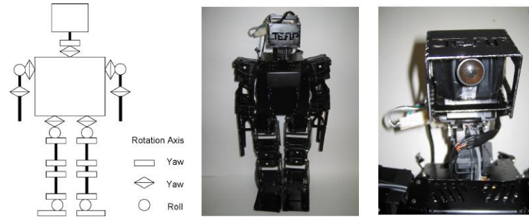
Fig. 1. The VisiON 4G robot: On the left side is a schematic overview of the actuators and their attitude in relation to the bodies. The middle and the right side figures are the front view of the whole body and the head part of the robot, respectively.
