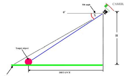
Fig. 9 Determination of the distance from the robot to the target object (Side View)
