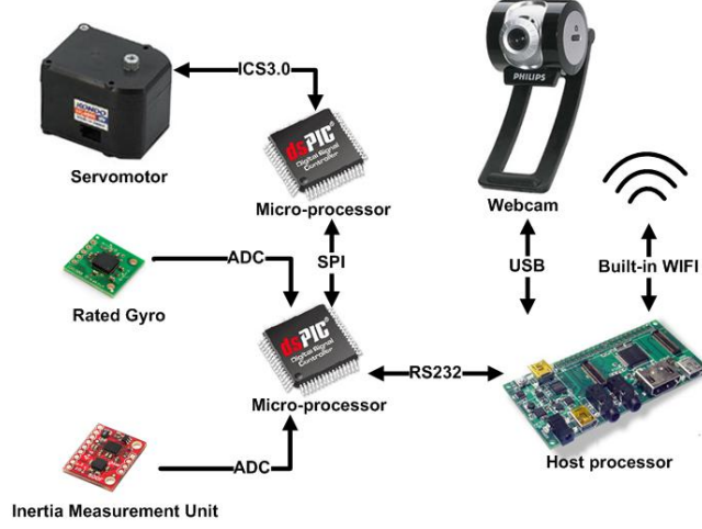
Fig. 2. Robo-Erectus Architecture
