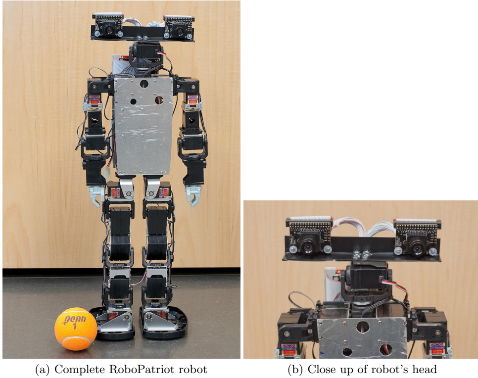
Fig. 1. 2010 RoboPatriot's robot and close up of stereo vision head and pan/tilt mount.
