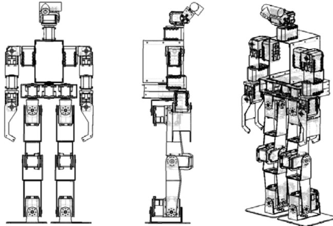
Fig. 2. Mechanical design of TWNHR-VI.
