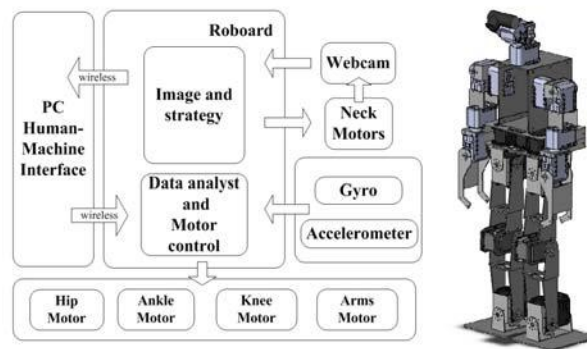
Fig. 3. Block diagram of TWNHR-VI's electrical system
