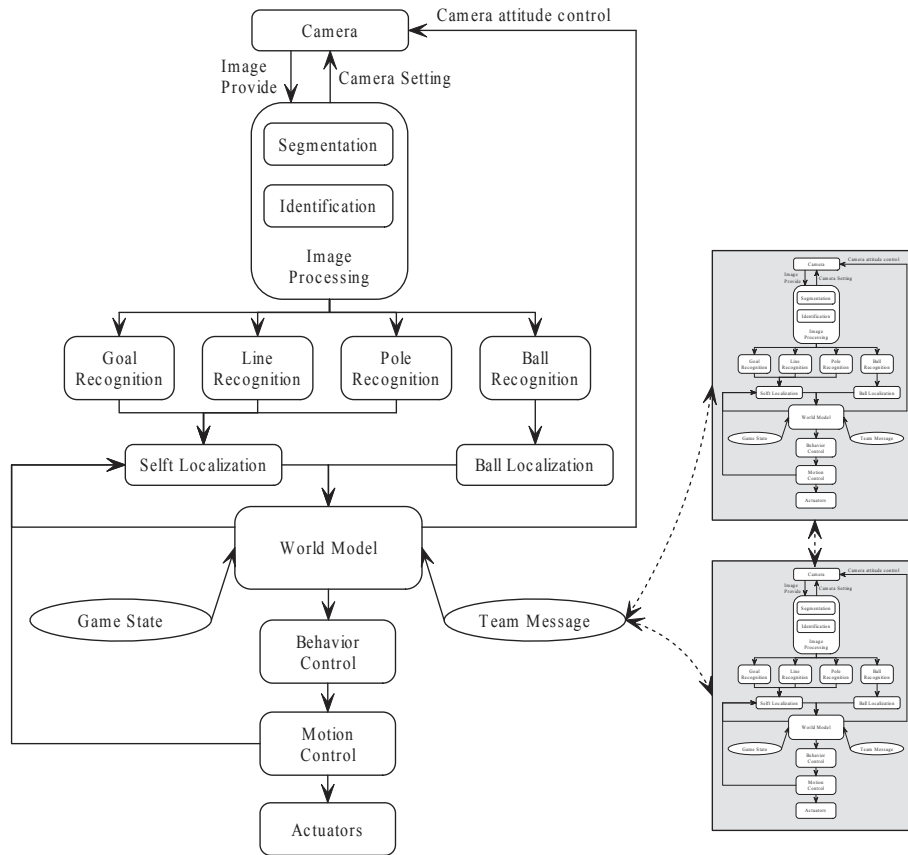
Fig. 5. Software Architecture
