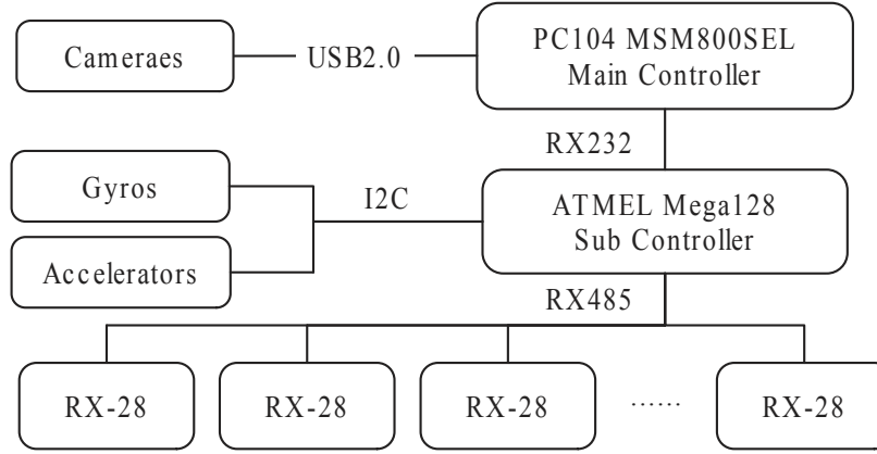
Fig. 4. Robot's Electrical Architecture
