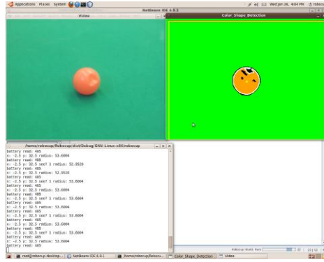
Fig. 2. Ball detection
