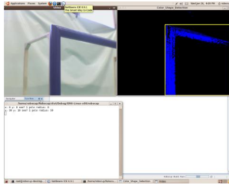
Fig. 3. Goal detection
