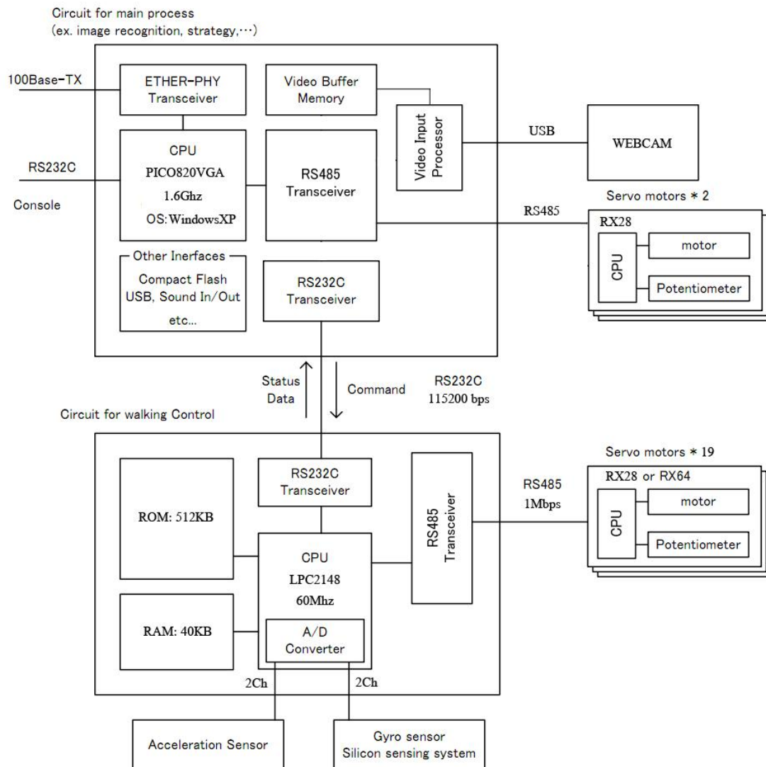
Fig.2: BSRU Architecture
