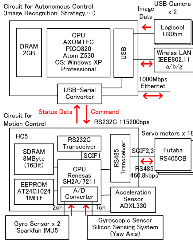
Fig.2 Overview of the Control System
