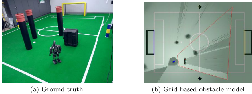
Fig. 3: Grid-based Obstacle Model: (a) shows a real world scene featuring multiple obstacles. (b) shows the grid-based obstacle model used on our robots.
