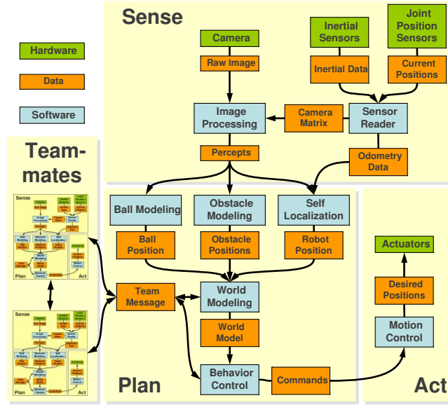
Fig. 2: An abstract overview of the implemented high level control architecture.
