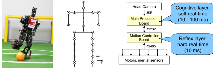
Fig. 1: Autonomous humanoid robot Bruno (©K. Binner) kicking a ball (left), kinematic robot structure (middle), main layers of information processing (right).
