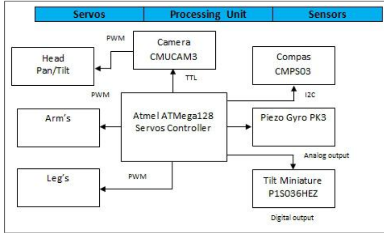
Fig. 2. Schematic electronic architecture of robots humanoids.
