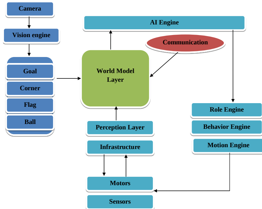
Fig.4. Software architecture.
