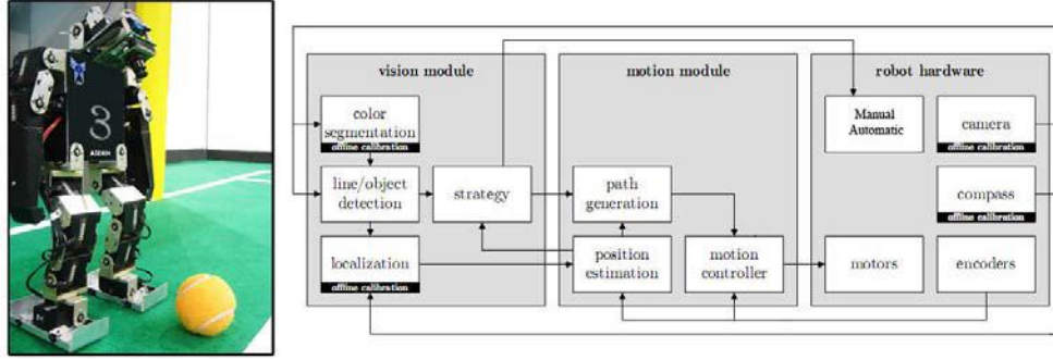
Fig. 2. (a) Our Humanoid soccer robot, (b) Overview of the Control System
