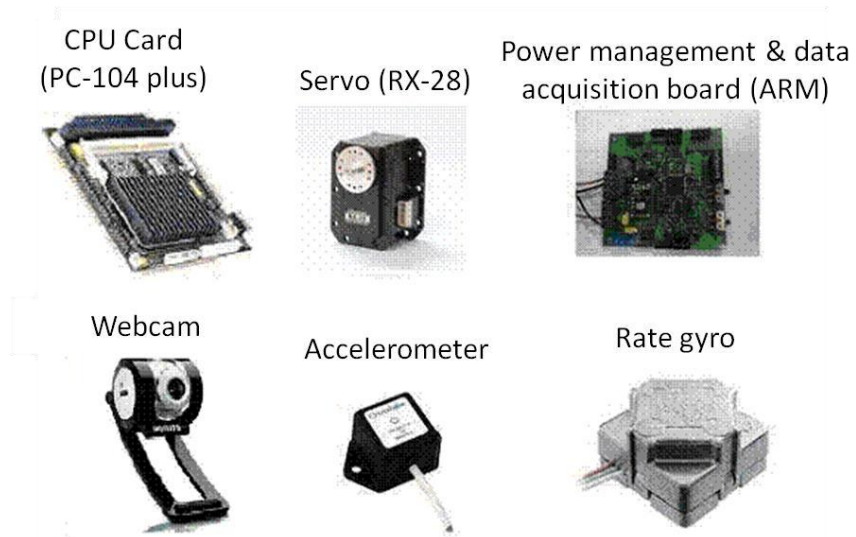
Fig. 2. Components of RO-PE-VI
