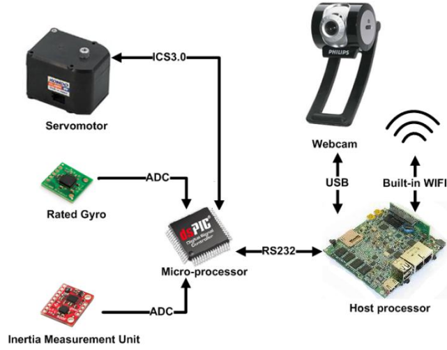
Fig. 2. Robo-Erectus Architecture
