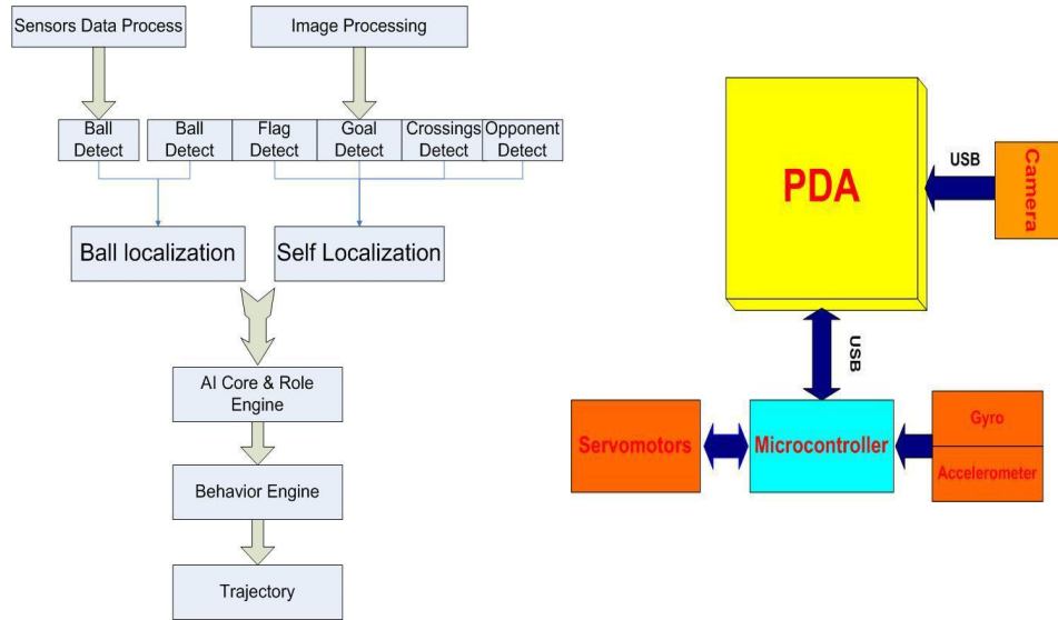
Fig. 2. Schematic of control architecture (right) and software flowchart (left).
