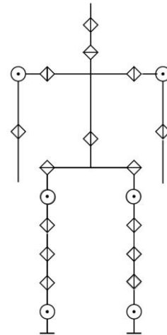
Fig 2. Kinematical Robot Structure
