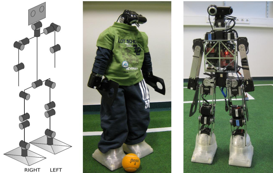
Fig. 1. Prototype of FUmoids 2012 model (middle/right) and its kinematics (left)
