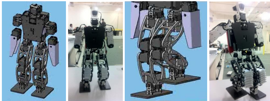
Fig. 1. Mechanical design and construction of the new robot.
