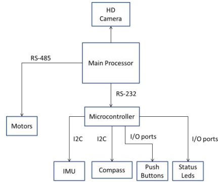
Fig. 2. Hardware architecture of the new Bogobots Platform.
