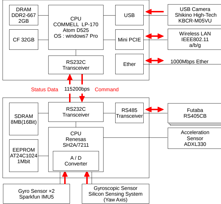
Fig.2 Overview of the Control System
