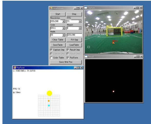
Fig.4 Graphic User Interface of Class Library "Local Vision"
