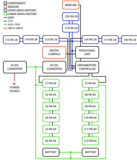
(a) Connection block diagram
