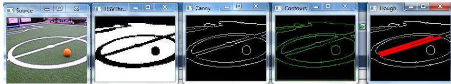
Fig. 3. Raw image with Canny edge detection and Hough transform.
