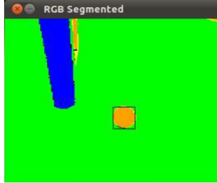
Fig. 2. Ball Detection.
