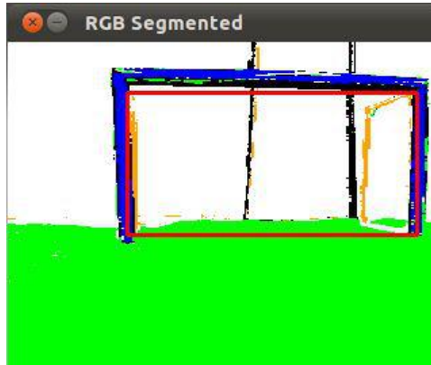
Fig. 3. Goal Detection.
