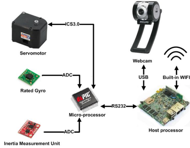
Fig. 2. Robo-Erectus Architecture
