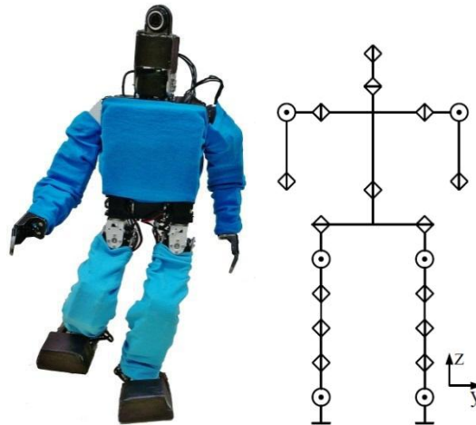
Figure 1. AUTMan “DROID2013” robot (left) and its kinematic
