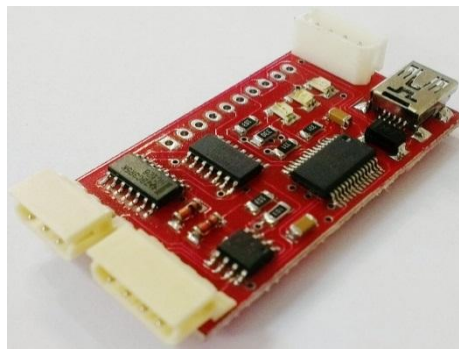
Figure 2. 9DOF IMU and RM-G146 sensor module
