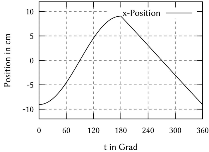
Fig. 3. The trajectory of the leg is based on a pendulum-like model: the passive dynamic walker. In the swingphase it acts like a pendulum (sinusoide). In the stance phase it moves linearly.
