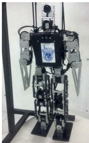
Fig. 1. Mechanical design and construction of Bogobot - 2.
