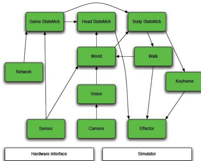
Fig. 3. Software architecture
