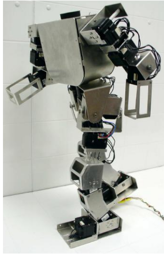
(a) DARwIn I
