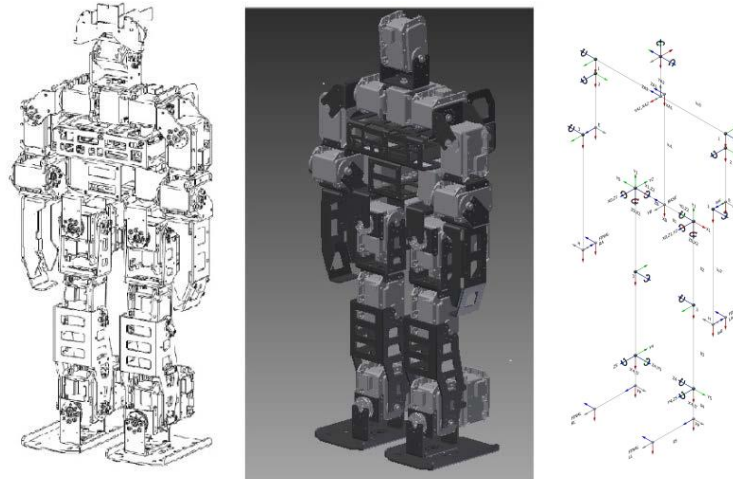
Fig. 2. Kinematic diagram of the dotMEX prototype.
