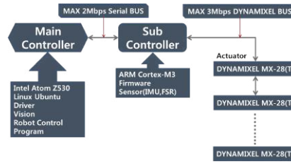
Fig. 2. Software architecture of KUbot
