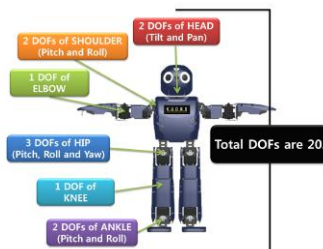
Fig. 1. Degree of freedom of KUBot
