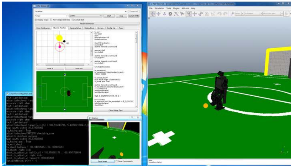
Fig.9 Simulator Software
