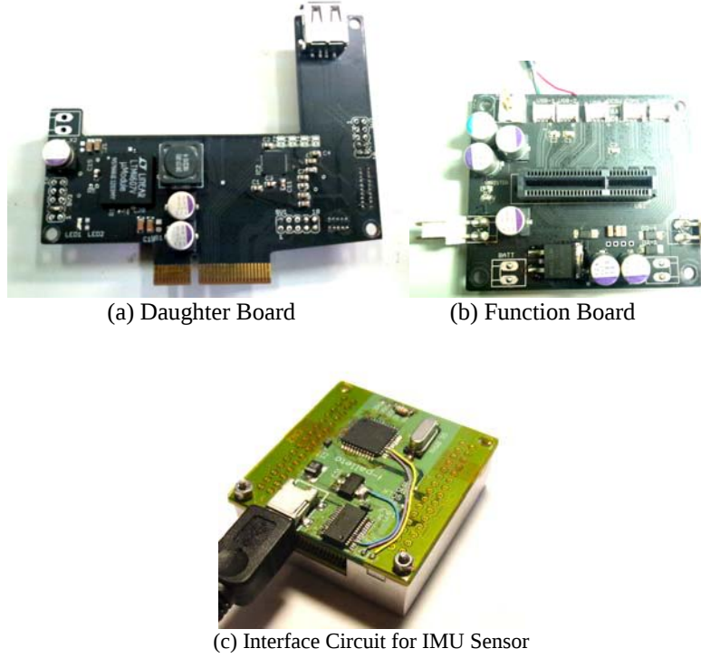
Fig.4. Developed Control Circuits
