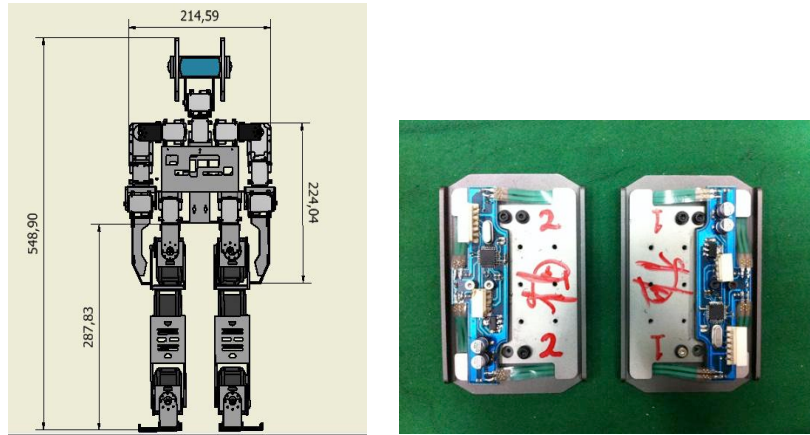
Figure 4. Mechanical dimensions and the FSR sensors on the soles of feet
