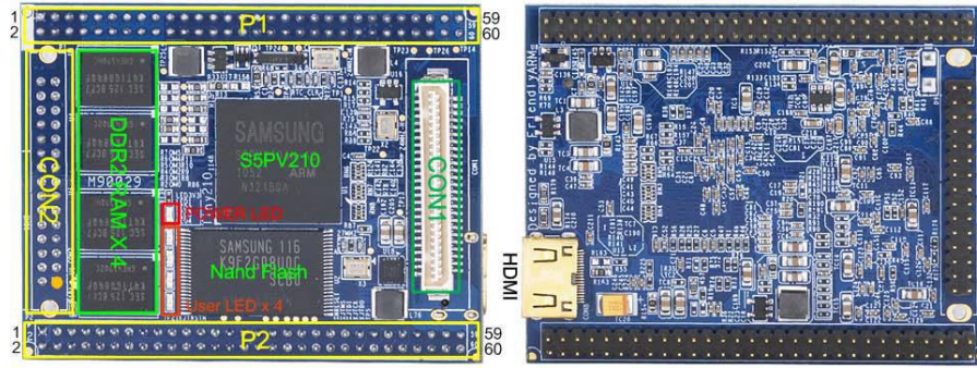
Fig. 2. Main Controller
