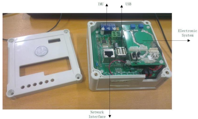
Fig. 3. Mother Board
